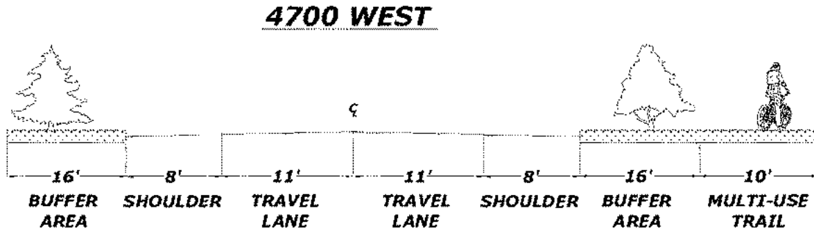
4700 West South - Proposed Roadway Cross-Section and Multi-Use Trail
